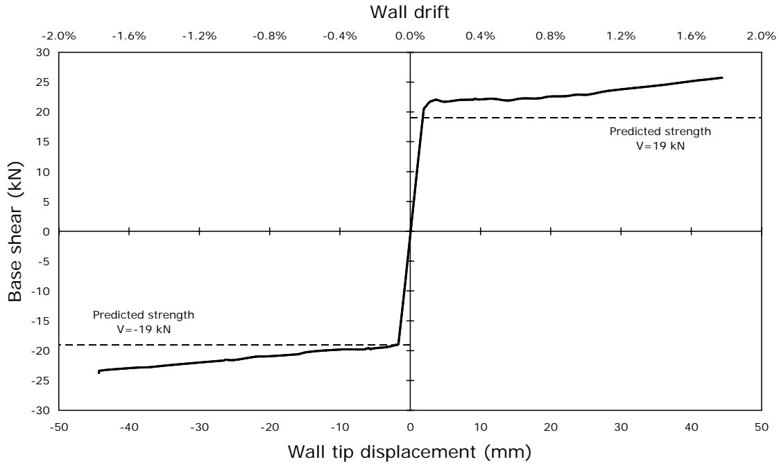
Figure 7: Force-displacement envelope
