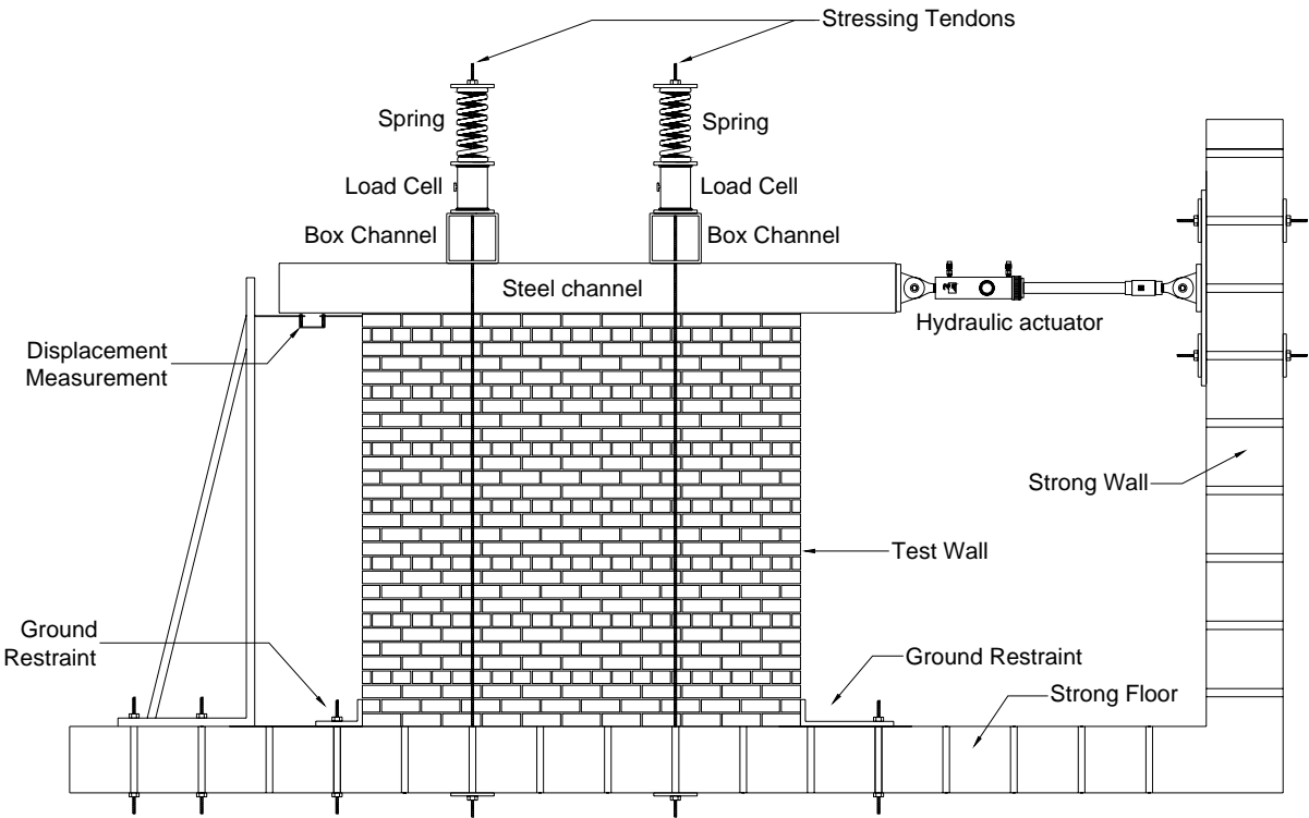
Figure 4: Test setup
