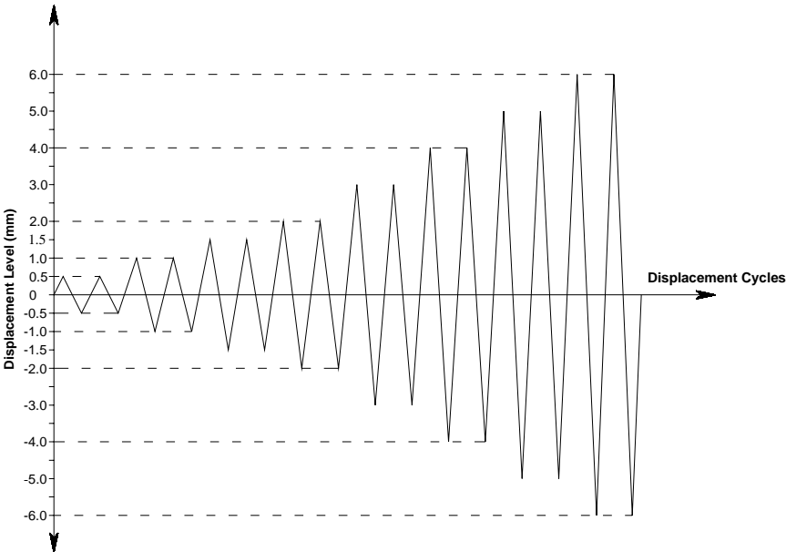
Figure 5. Displacement cycles
