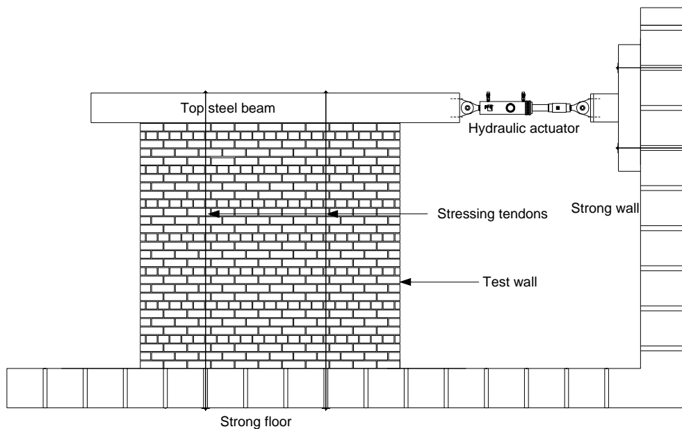
Figure 4. Test Setup
