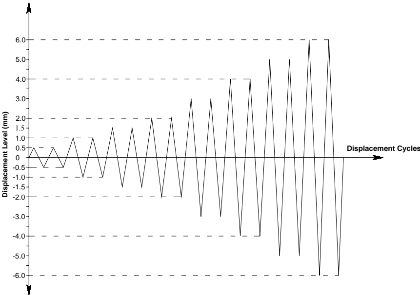
Figure 5. Displacement cycles
