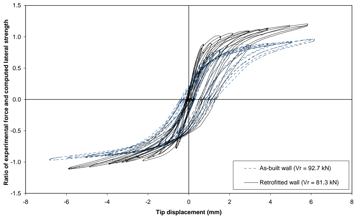
Figure 6. Ratio of the experimental force and computed lateral strength versus tip displacement
